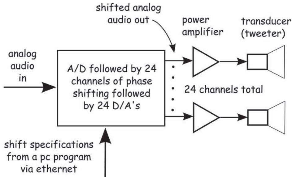
Fig. 8. High-level overview of the phase-shift array system.
