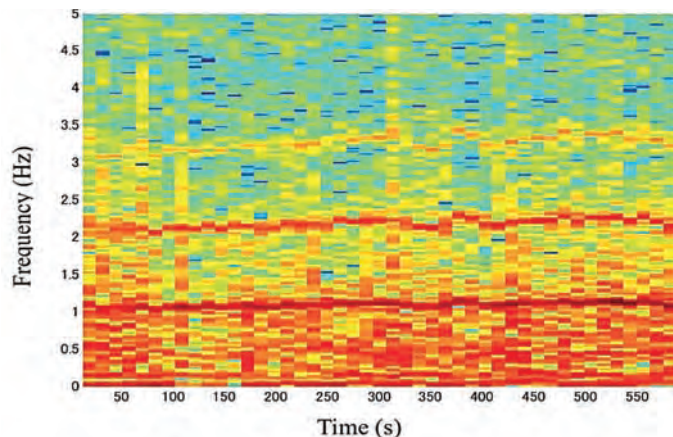
Fig. 7. Spectrum of infrasonic pressure in the occluded ear canal.
