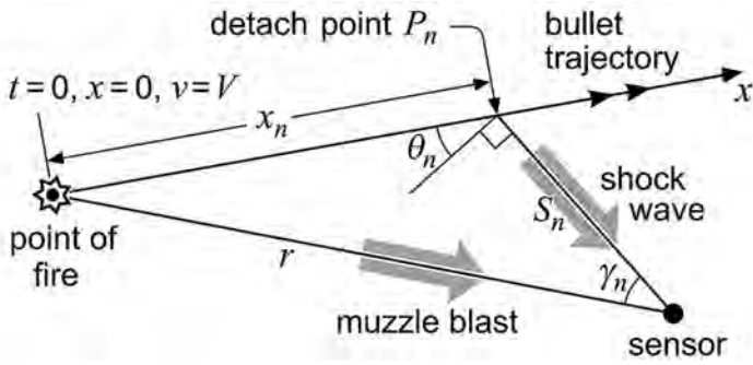
Fig. 7. Acoustic transient signals—the muzzle blast is generated at the point of fire and the ballistic shock wave originates from the detach point along the bullet’s trajectory.
