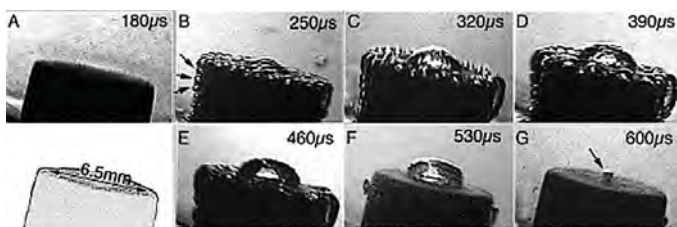
Fig. 11. Comparison of measured 36 and simulated bubble cluster collapse 44 at the distal face of a cylindrical model stone. The model can capture the complex cloud behavior around a stone, and potentially be used to test parameters, for example to maximize the pressure generated in the stone at collapse. Reprinted with permission from Journal of Endourology and IEEE. (© IEEE)
