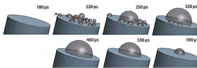
Fig. 11. Comparison of measured 36 and simulated bubble cluster collapse 44 at the distal face of a cylindrical model stone. The model can capture the complex cloud behavior around a stone, and potentially be used to test parameters, for example to maximize the pressure generated in the stone at collapse. Reprinted with permission from Journal of Endourology and IEEE. (© IEEE)
