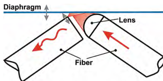
Fig. 1. Schematic construction principle of the optical microphone with lenses on the fibers. A constant intensity low noise light source emits light to the back of the microphone diaphragm via the transmitting fiber. The excursion of the microphone diaphragm then yields to a modulation of the light intensity in the receiving fiber (left).
