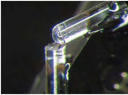
Fig. 2. Transmitting optical fiber with lens (top) and receiving fiber without lens (bottom) fixed in the carrier frame (right). For better visibility the diaphragm was not mounted yet.
