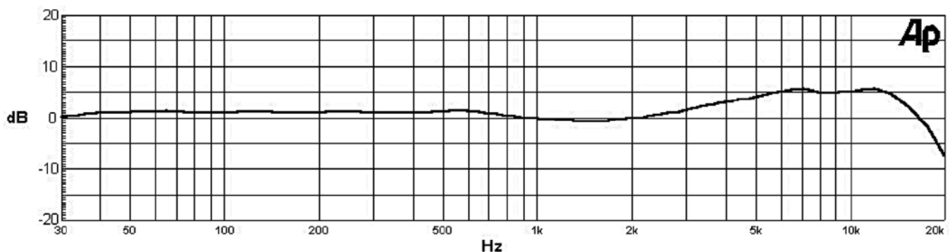
Fig. 4. Relative frequency response of the optical microphone.
